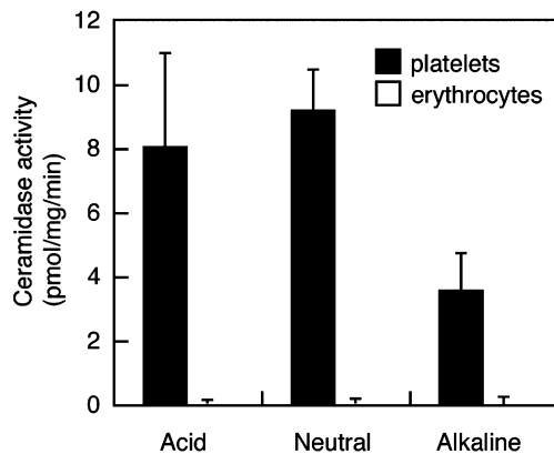
Fig. 4. Absence of ceramidase in erythrocytes. Total cell lysates (50 \mu\text{g} protein) prepared from platelets or erythrocytes were incubated with 27.5 \mu\text{M} \text{C}_{12} -NBD-ceramide for 3 h at 37^\circ\text{C} at pH 4.5 (acid), pH 7.5 (neutral), or pH 9.4 (alkaline). Lipids were extracted and separated by TLC. The amount of NBD-dodecanoic acid was quantified using a fluorimaging analyzer FLA-2000. Values shown represent the means \pm SD from three independent experiments.
