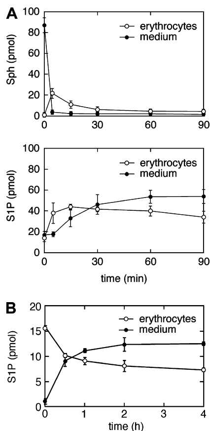
Fig. 2. Constitutive release of S1P from erythrocytes. (A) Erythrocytes ( 10^8 cells in 100 \mu\text{l} ) were treated with 1 \mu\text{M} (100 pmol) Sph and incubated at 37 °C. At 0, 5, 15, 30, 60, or 90 min, erythrocytes were separated from the medium by centrifugation. Total lipids were prepared from both medium and erythrocytes, and Sph (upper panel) and S1P (lower panel) amounts were quantified by HPLC. Values shown represent the means \pm SD from four independent experiments. (B) Erythrocytes ( 10^8 cells in 100 \mu\text{l} ) were prepared at 4 °C and incubated at 37 °C for the indicated time periods. Erythrocytes were separated from the medium by centrifugation, and total lipids were prepared from both medium and erythrocytes. S1P levels were quantified by HPLC. Values shown represent the means \pm SD from three independent experiments.
